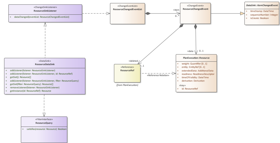
Figure 10.27 ResourceDataSink (Class diagram)
