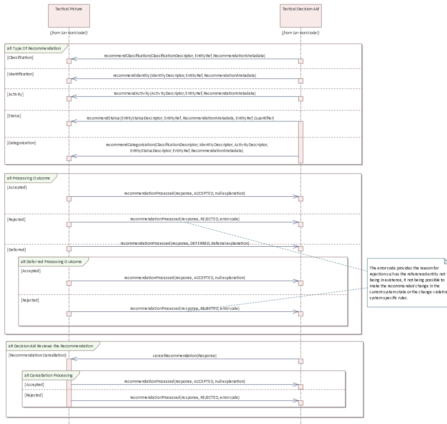
Figure 10.46 TacticalPictureRecommendations - Categorization - Alternate Flow (Interaction diagram)
