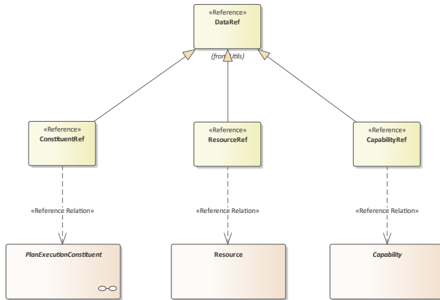
Figure 9.11 Reference DataTypes (Class diagram)
