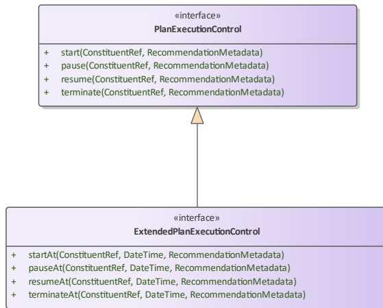
Figure 10.35 ActionControlRecommendation (Class diagram)
