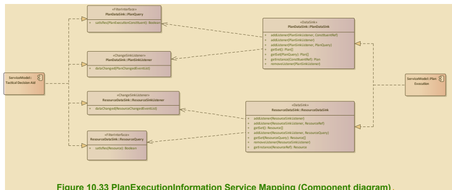
Figure 10.33 PlanExecutionInformation Service Mapping (Component diagram)
