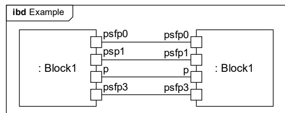
Figure 13: Connectors in Figure 12 replaced or added between ports added in Subclauses 9.4.3.2 and 9.4.3.3
