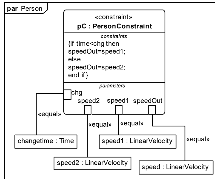
Figure 119: Parametric diagram applying the person constraint
