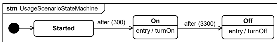
Figure 95: Humidifier Usage Scenario State Machine Diagram
