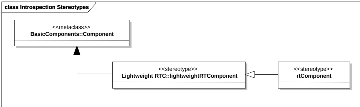
Figure 5.32 - Introspection Stereotypes
