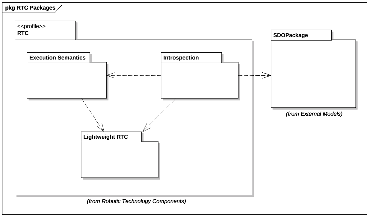
Figure 1.1 - RTC packages
