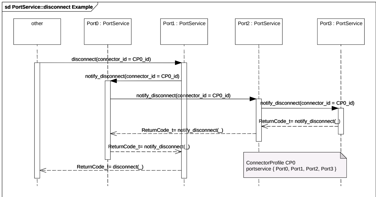
Figure 5.34 - PortService::disconnect Example
