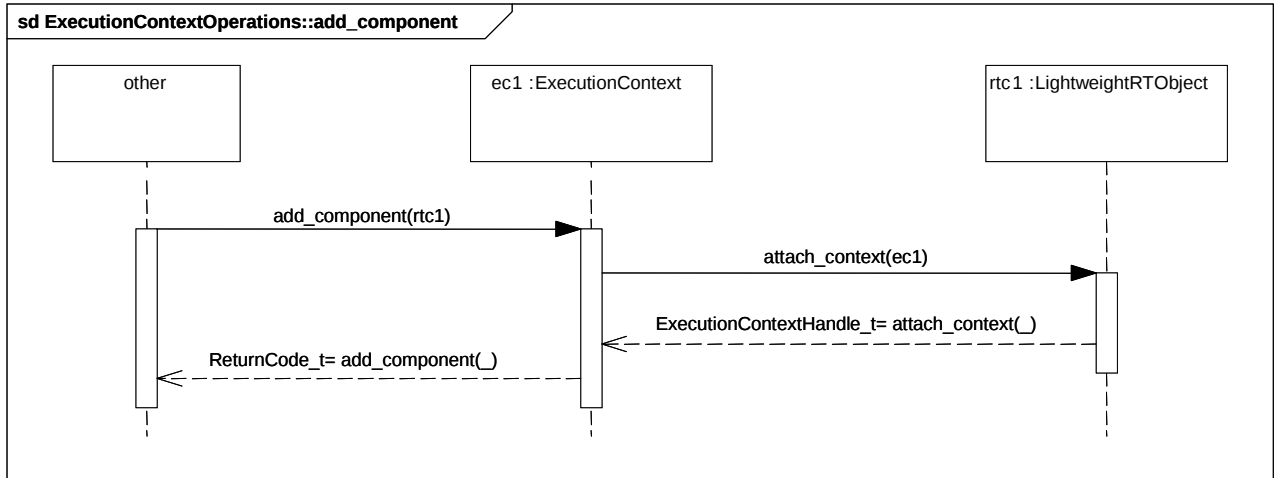
Figure 5.10 - ExecutionContextOperations::add_component
