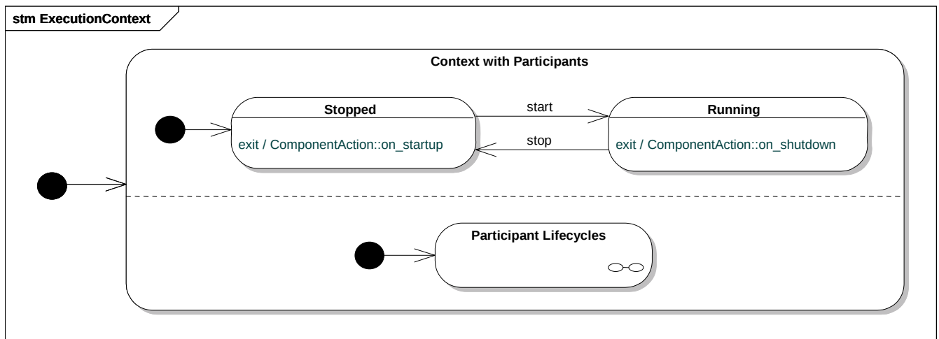
Figure 5.7 - ExecutionContext
