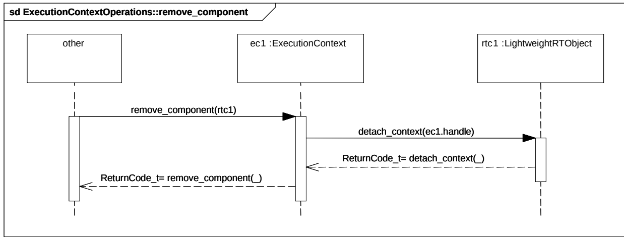
Figure 5.11 - ExecutionContextOperations::remove_component
