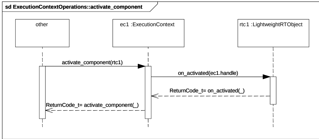
Figure 5.12 - ExecutionContextOperations::activate_component
