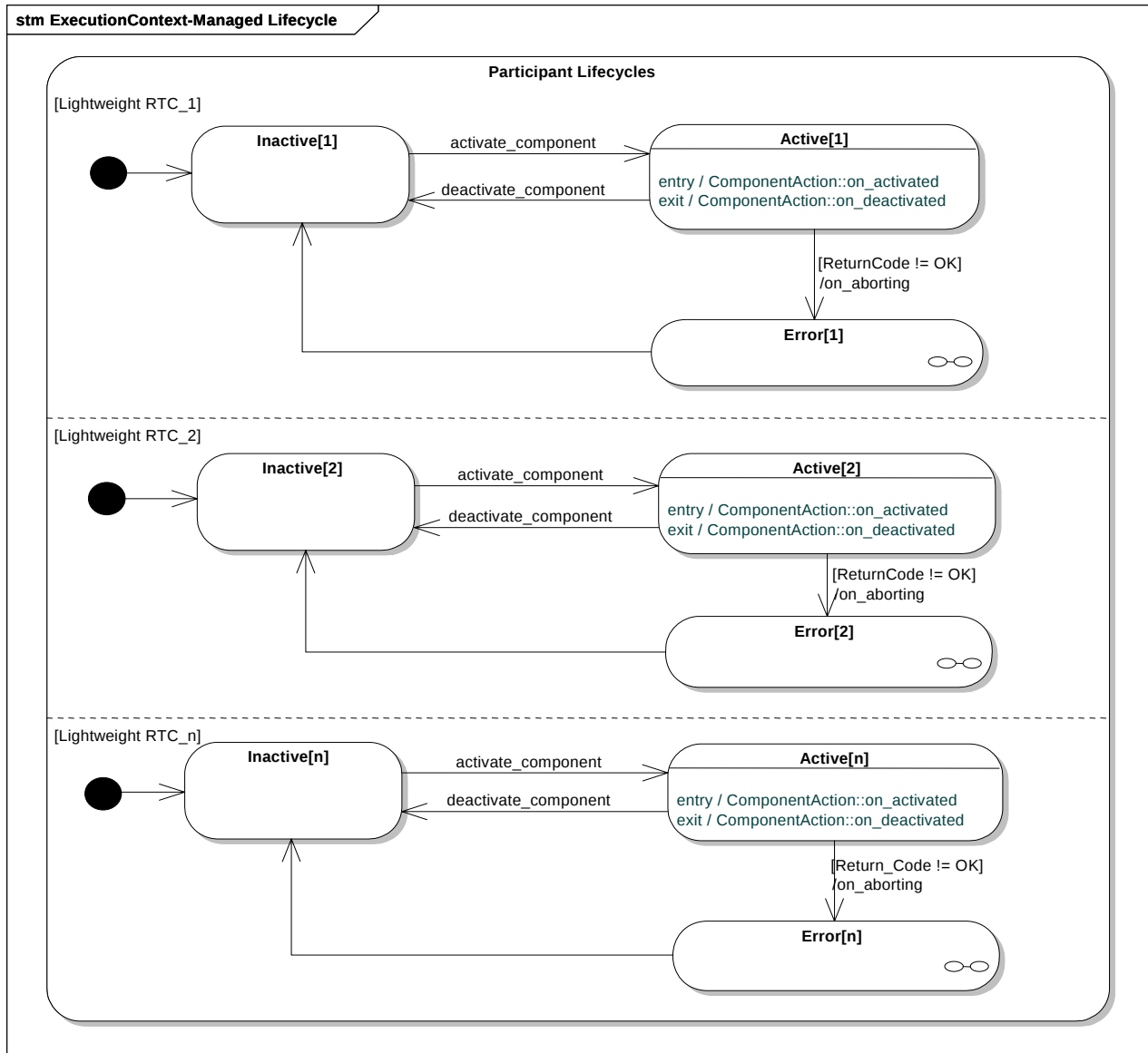
Figure 5.5 - ExecutionContext-Managed Lifecycle
