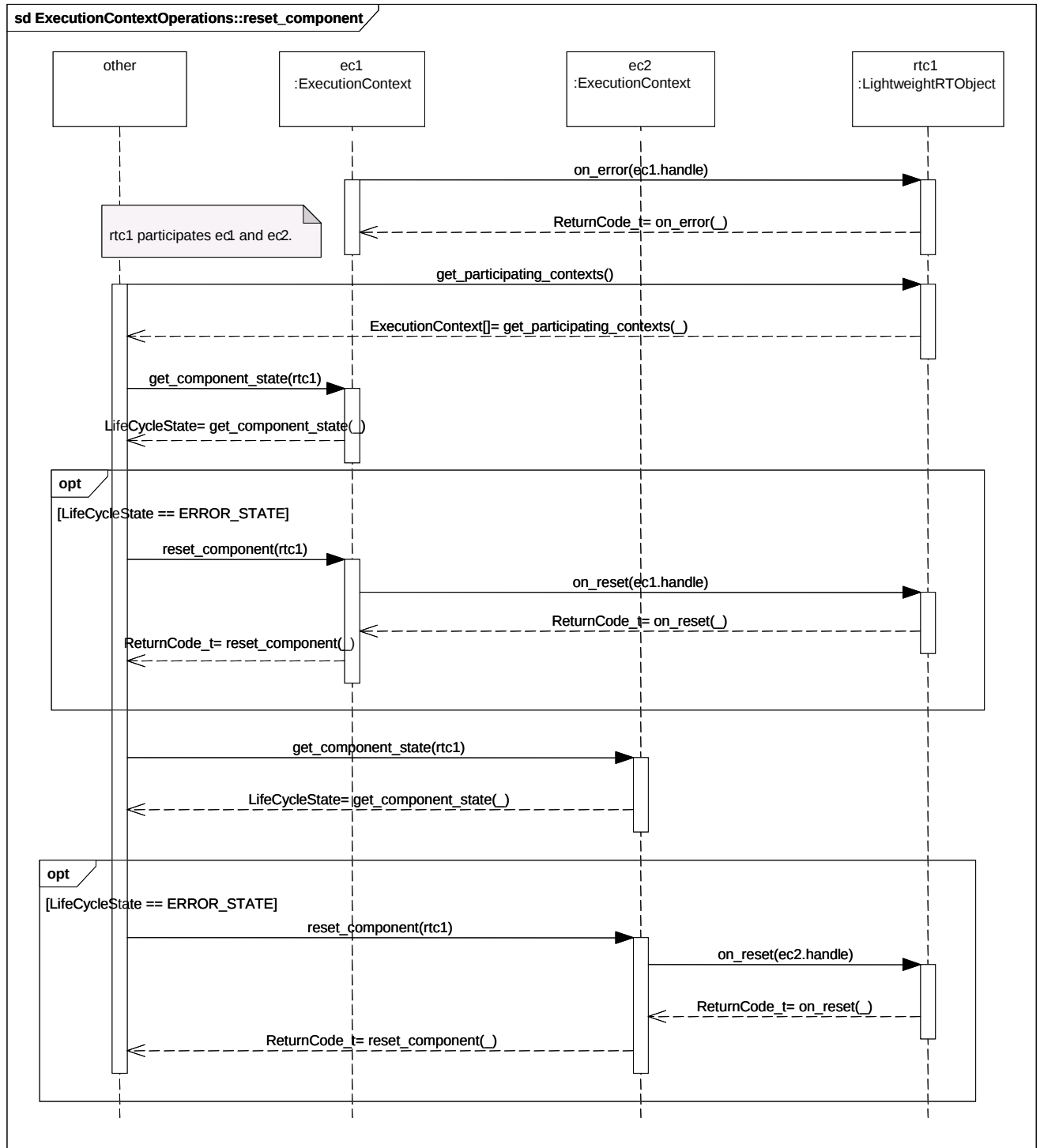
Figure 5.14 - ExecutionContextOperations::reset_component
