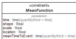
Figure 9.219 – MeanFunction
