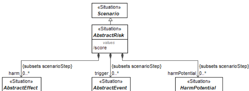
Figure 9.23 – AbstractRisk
