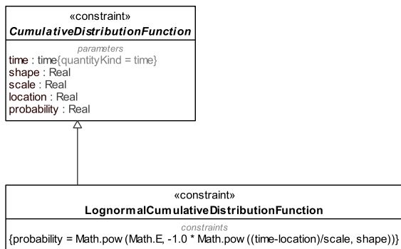
Figure 9.218 – LognormalCumulativeDistributionFunction
