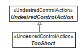
Figure 9.102 – TooShort
