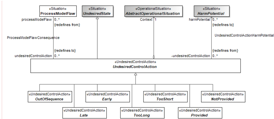
Figure 9.111 – UndesiredControlAction
