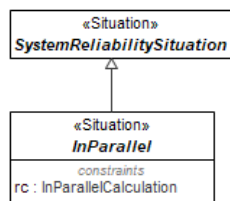
Figure 1.201 - InParallel
