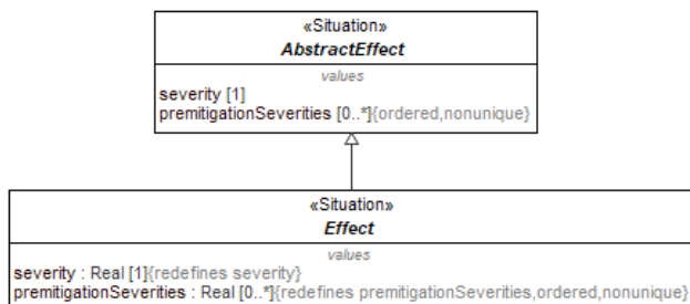
Figure 9.16 – Effect
