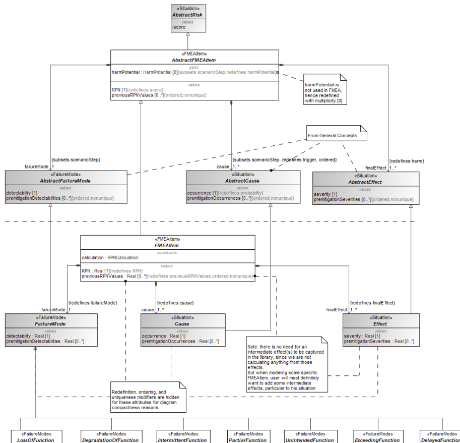
Figure 10.7 – FMEA Library
