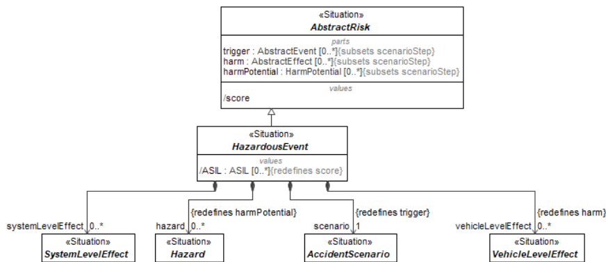
Figure 9.160 – HazardousEvent
