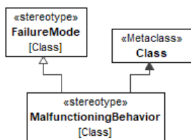
Figure 9.173 – MalfunctioningBehavior
