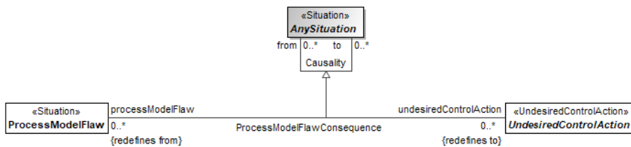
Figure 9.114 – ProcessModelFlawConsequence
