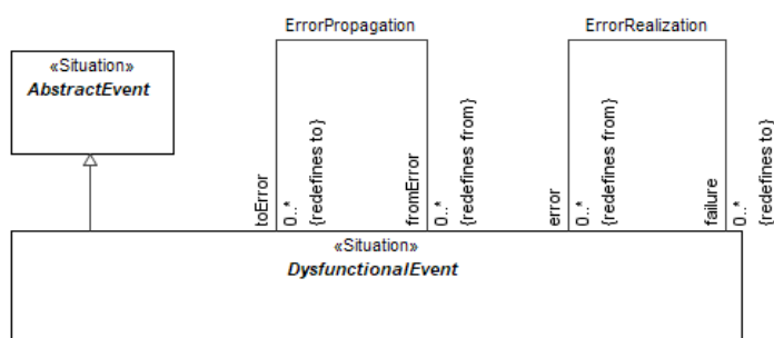
Figure 9.12 – DysfunctionalEvent
