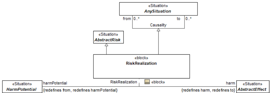
Figure 9.112 – RiskRealization
