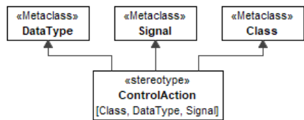
Figure 9.116 – ControlAction
