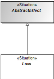
Figure 9.26 – Loss
