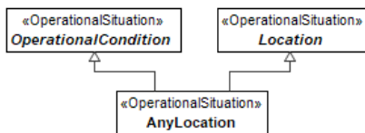
Figure 9.168 – AnyLocation
