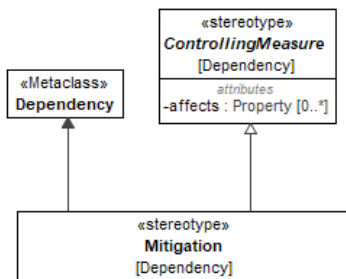
Figure 9.33 – Mitigation
