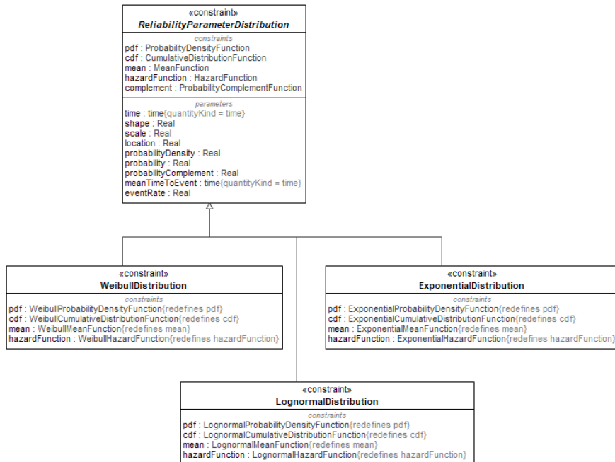
Figure 0.30 - Distributions
