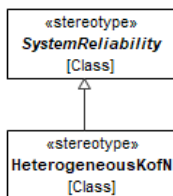
Figure 9.242 – HeterogeneousKofN
