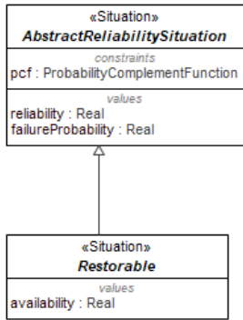
Figure 1.193 - Restorable Attributes
