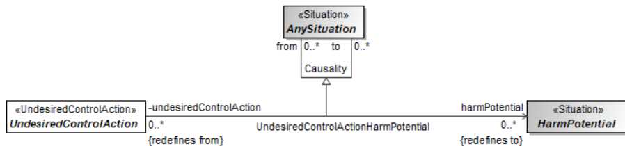
Figure 9.115 – UndesiredControlActionHarmPotential
