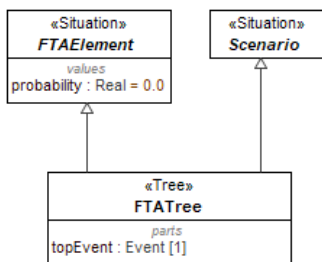
Figure 9.61 – FTATree
