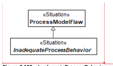
Figure 9.109 – InadequateProcessBehavior
