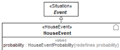
Figure 9.69 – HouseEvent
