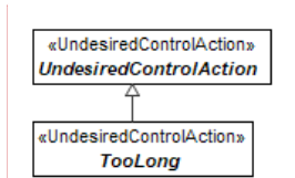
Figure 9.101 – TooLong
