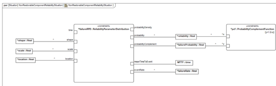
Figure 0.33 - NonRestorableComponentReliabilitySituation
