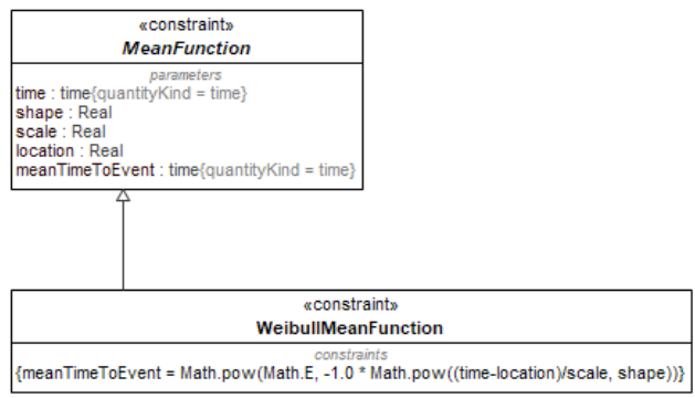
Figure 9.221 – WeibullMeanFunction
