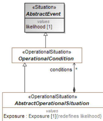
Figure 9.146 – AbstractOperationalSituation
