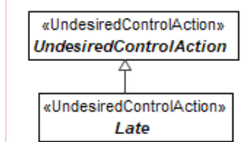
Figure 9.99 – Late
