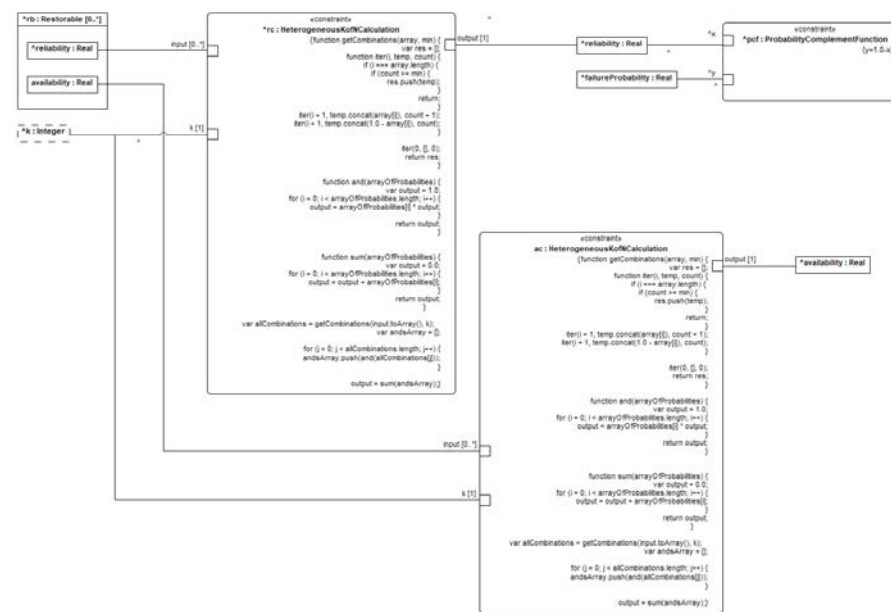
Figure 0.29 - RestorableHeterogeneousKofN
