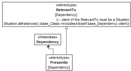
Figure 9.38 – PresentIn
