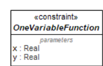
Figure 9.207 – OneVariableFunction
