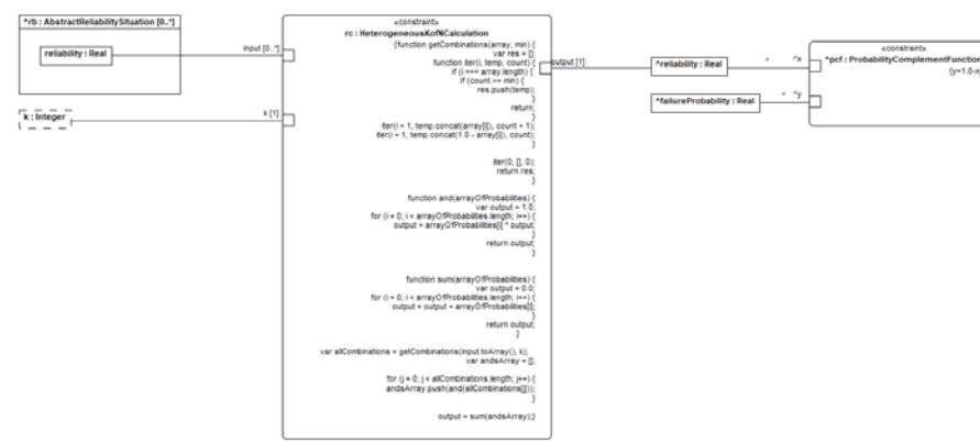
Figure 0.28 - HeterogeneousKofN
