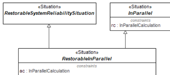
Figure 1.202 - RestorableInParallel
