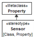
Figure 9.122 – Sensor
