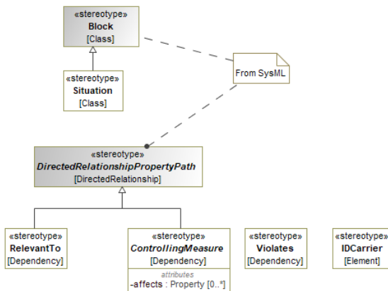
Figure 10.2 – CoreProfile
