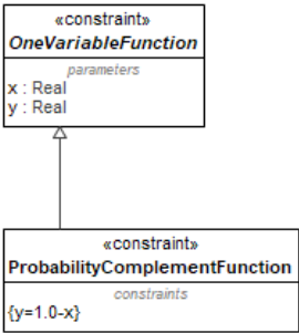
Figure 9.208 – ProbabilityComplementFunction
