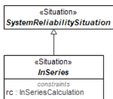
Figure 1.199 - InSeries Attributes
