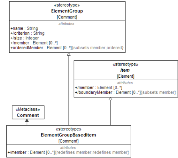
Figure 9.40 – ElementGroupBasedItem
