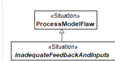
Figure 9.110 – InadequateFeedbackAndInputs
