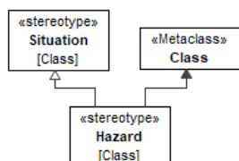
Figure 9.36 – Hazard
