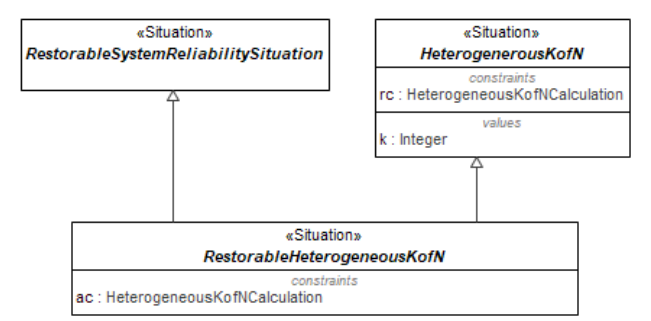
Figure 1.206 - RestorableHeterogeneousKofN
