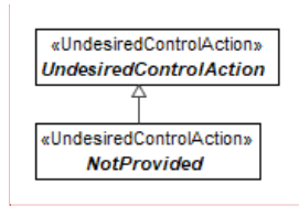
Figure 9.104 – NotProvided
