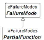
Figure 9.55 – PartialFunction
