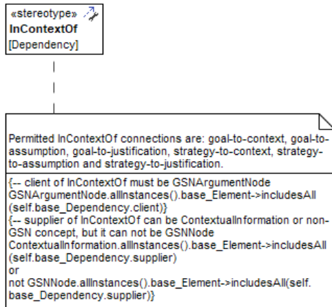
Figure 9.138 – InContextOf
