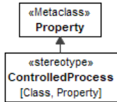
Figure 9.120 – ControlledProcess
