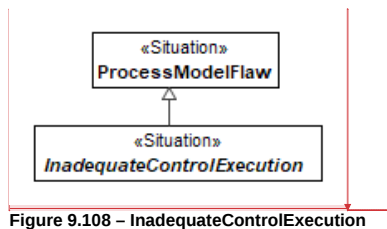
Figure 9.108 – InadequateControlExecution
