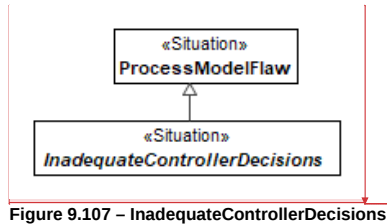
Figure 9.107 – InadequateControllerDecisions
