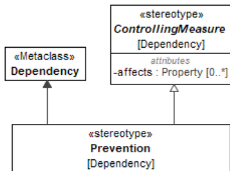
Figure 9.32 – Prevention
