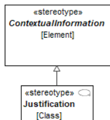
Figure 9.137 – Justification
