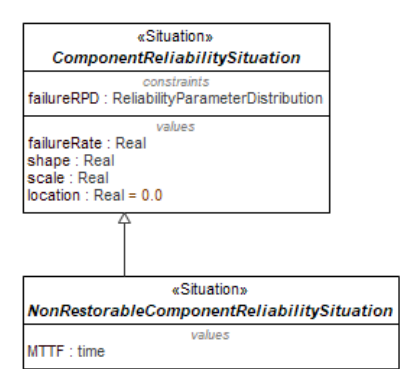
Figure 1.196 - NonRestorableComponentReliabilitySituation
