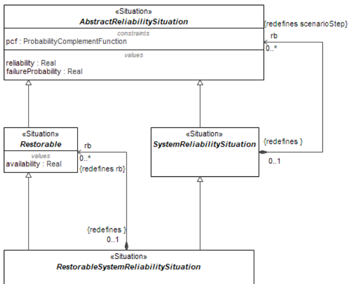
Figure 1.198 - RestorableSystemReliabilitySituation Attributes
