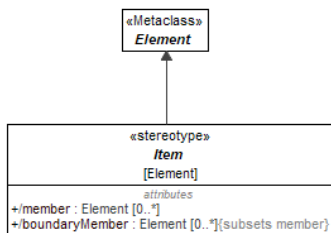
Figure 9.37 – Item
