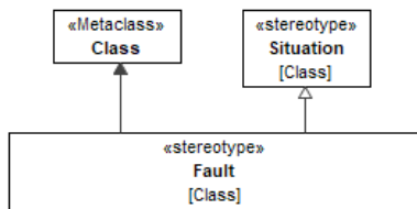
Figure 9.30 – Fault
