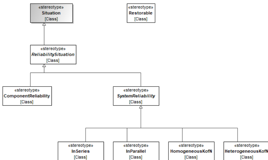
Figure 0.32 - RBD Profile
