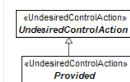
Figure 9.103 – Provided
