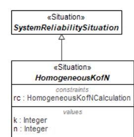
Figure 1.203 - HomogeneousKofN
