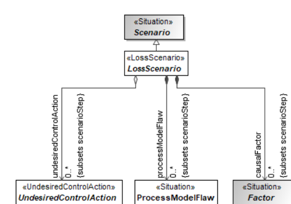
Figure 9.105 – LossScenario
