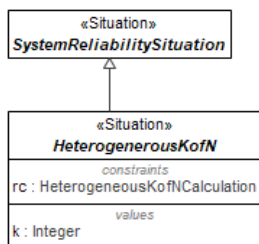
Figure 1.205 - HeterogeneousKofN
