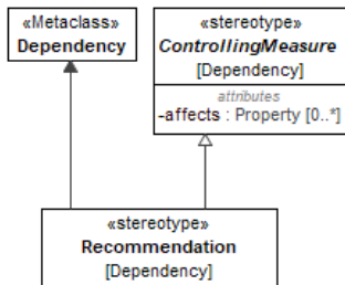
Figure 9.34 – Recommendation
