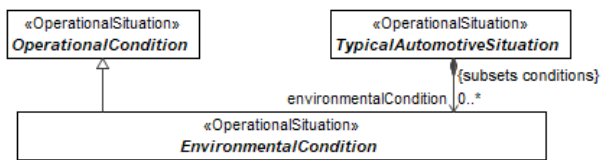
Figure 9.144 – EnvironmentalCondition
