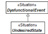
Figure 9.24 – UndesiredState
