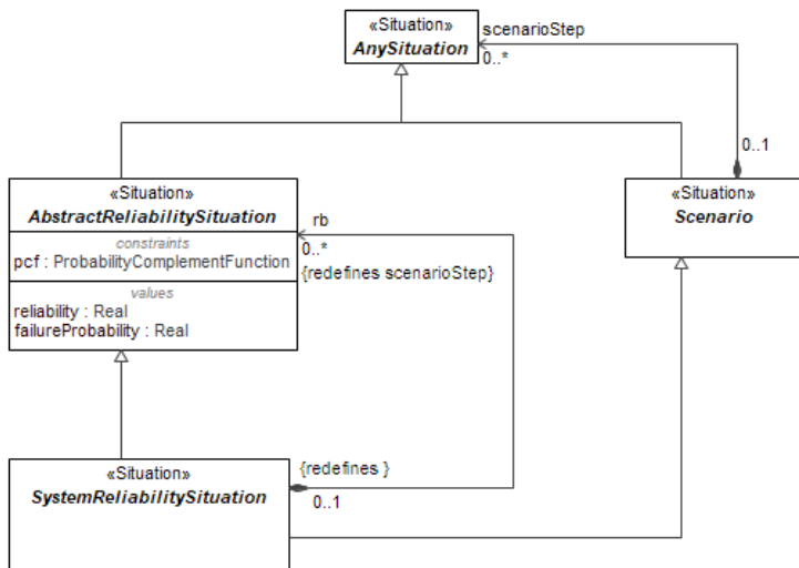
Figure 1.197 - SystemReliabilitySituation Attributes
