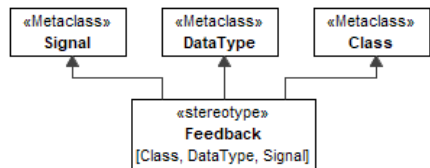
Figure 9.117 – Feedback
