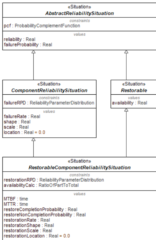
Figure 1.195 - RestorableComponentReliabilitySituation Attributes
