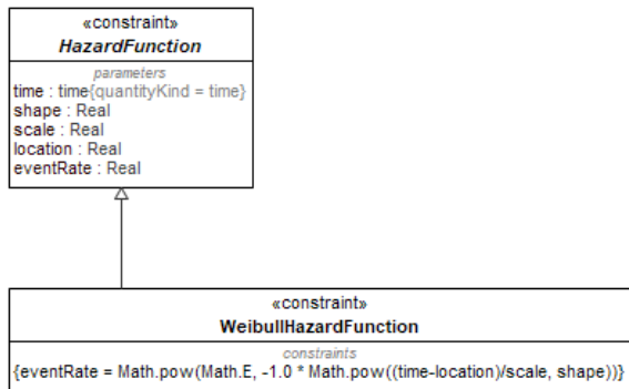
Figure 9.225 – WeibullHazardFunction
