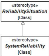
Figure 9.238 –SystemReliability
