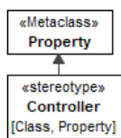
Figure 9.123 – Controller
