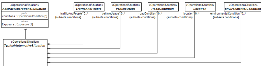
Figure 9.147 – TypicalAutomotiveSituation
