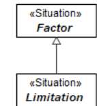
Figure 9.25 – Limitation
