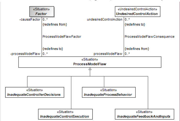
Figure 9.106 – ProcessModelFlaw
