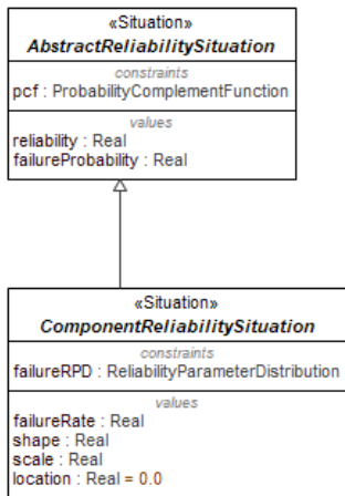
Figure 1.194 - ComponentReliabilitySituation
