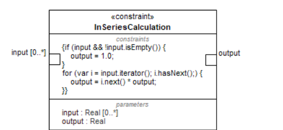
Figure 9.231 – InseriesCalculation
