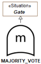
Figure 9.78 – MAJORITY_VOTE
