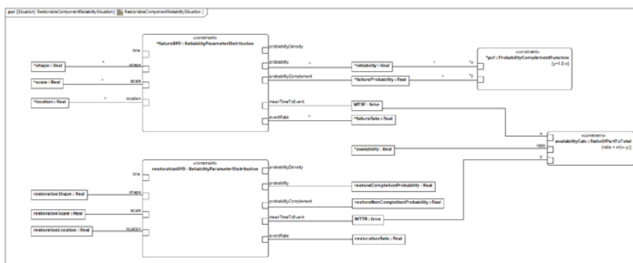
Figure 0.34 - RestorableComponentReliabilitySituation
