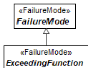
Figure 9.57 – ExceedingFunction
