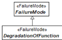
Figure 9.53 – DegradationOfFunction
