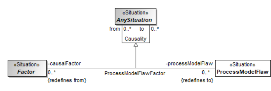
Figure 9.113 – ProcessModelFlawFactor
