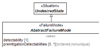
Figure 9.13 – AbstractFailureMode
