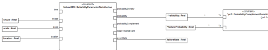
Figure 0.21 - ComponentReliabilitySituation
