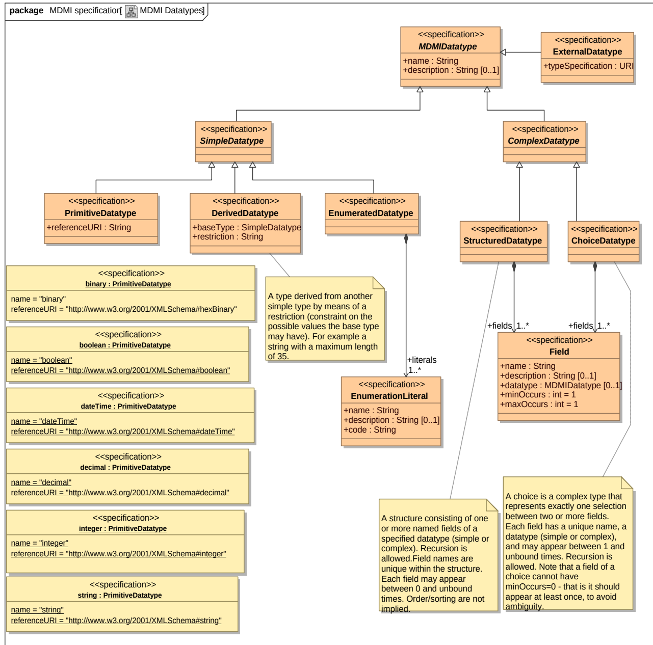
Figure 8.4.2 – Complex Datatype
