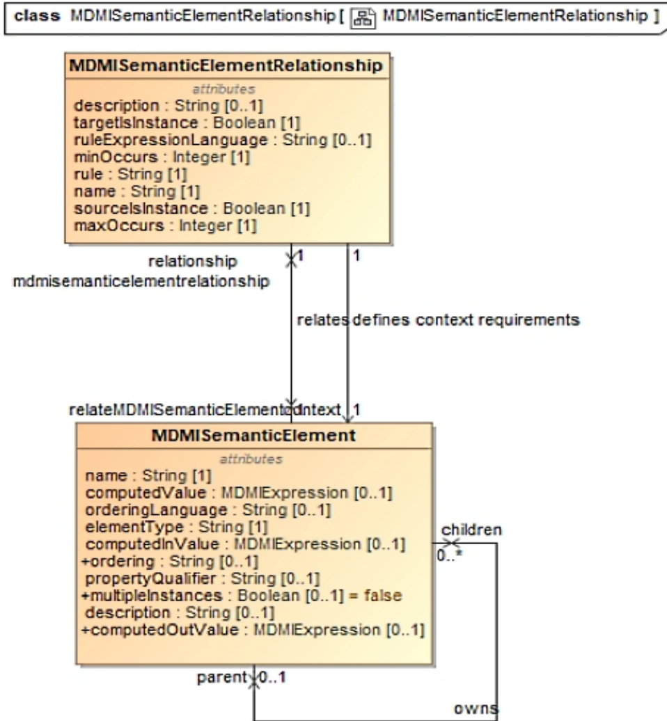
Figure 8.6 – MDMISemanticElementRelationship
