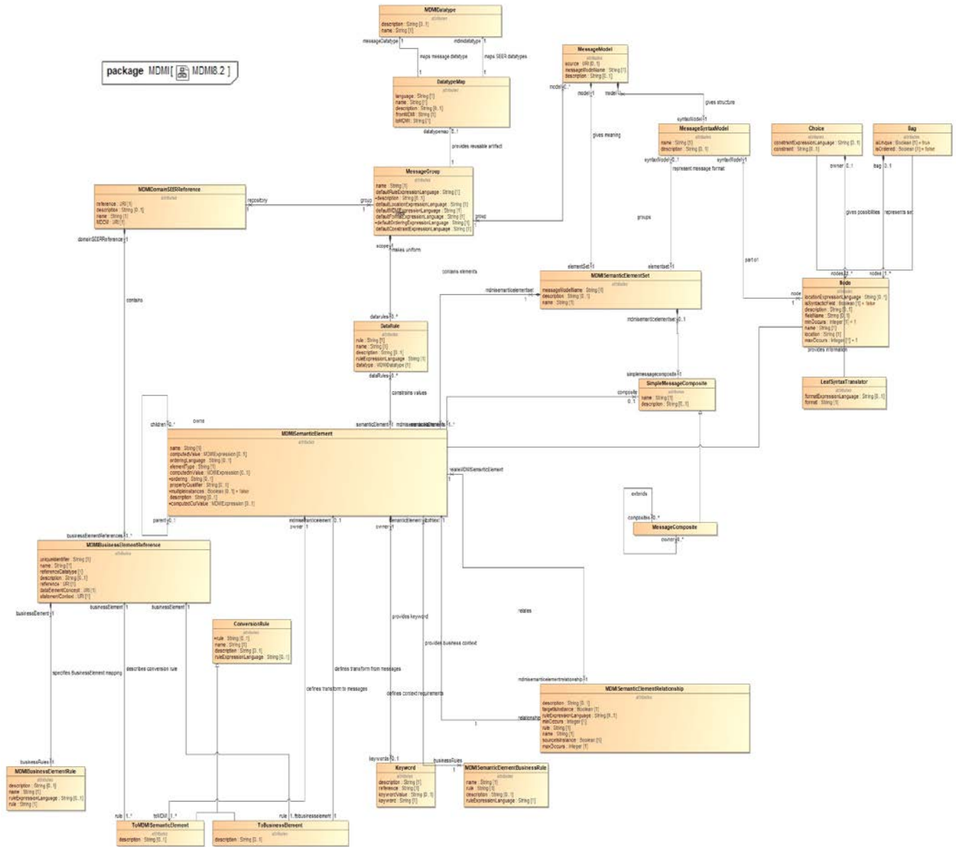
Figure 8.8 – Summary: Complete Metamodel
