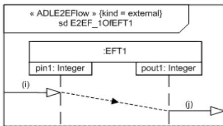
Figure A.20. Example of an EAST-ADL2 external end-to-end flow for an elementary ADLFunctionType
