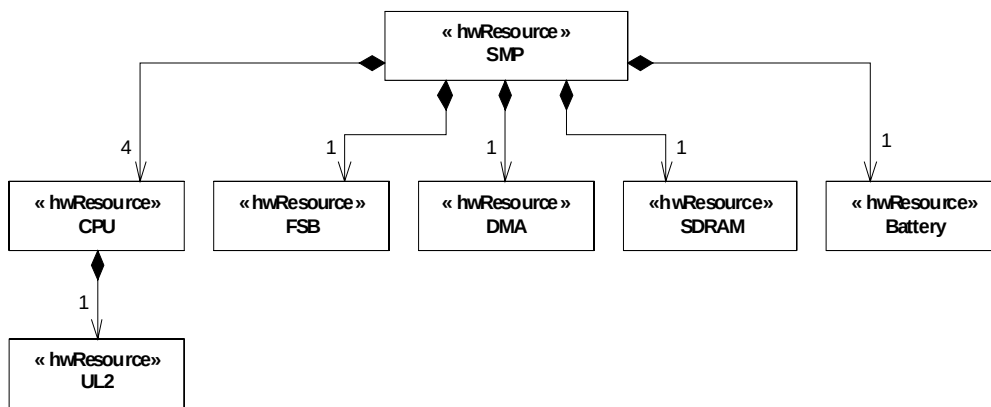
Figure 14.77 - SMP description
