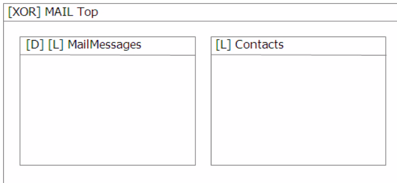
Figure A.5 - IFML model of the Top Container of the email application
