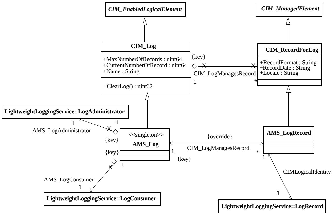
Figure 7.6 - Log class
