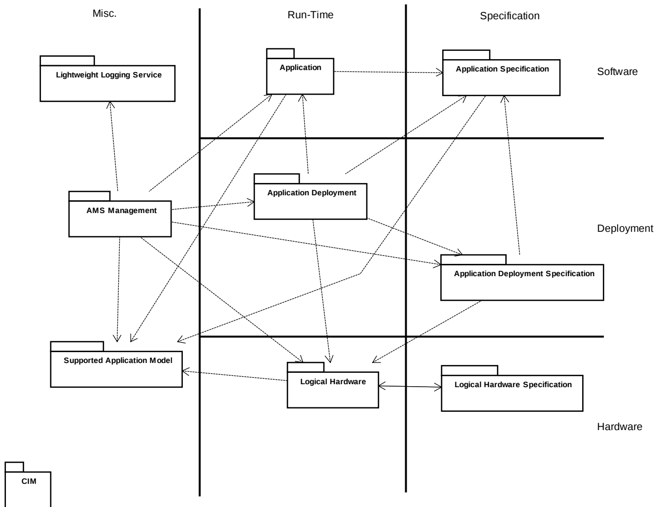
Figure 7.2 - Packages
