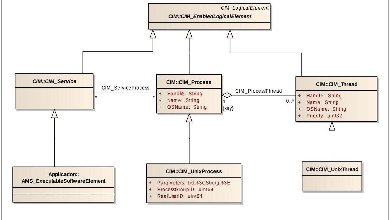
Figure 7.9 - Application class diagram (3/3)
